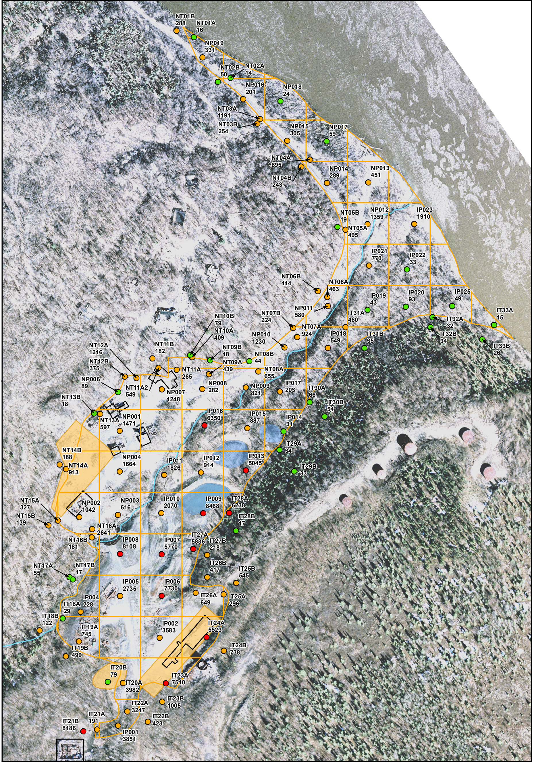
Figure 3-8 2010 Limited Sampling Event XRF Screening Results Arsenic
